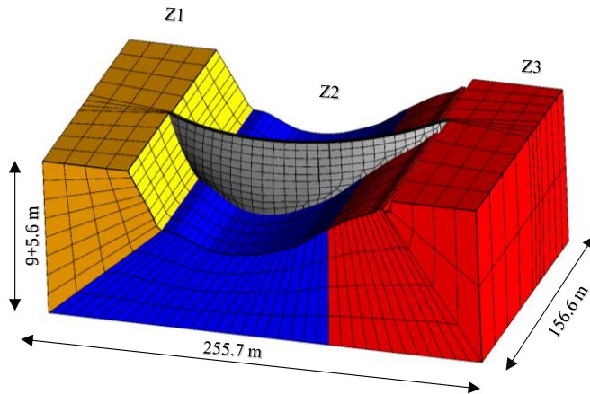
a) 2 nd order 20 node brick isoparametric elements representing the dam and its foundation (Z1 – Left bank, Z2 – Valley bottom and Z3 – Right bank)
