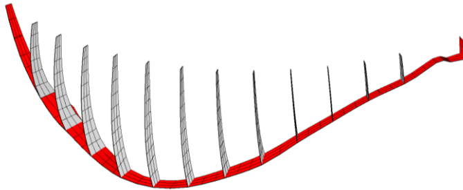
b) 2 nd order 8x8 node joint interface finite elements representing the dam/foundation interface and the contraction joints.
